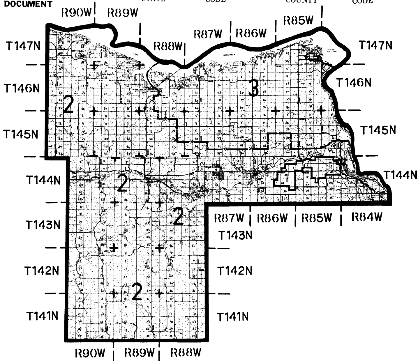
SECTIONIZED TOWNSHIP
